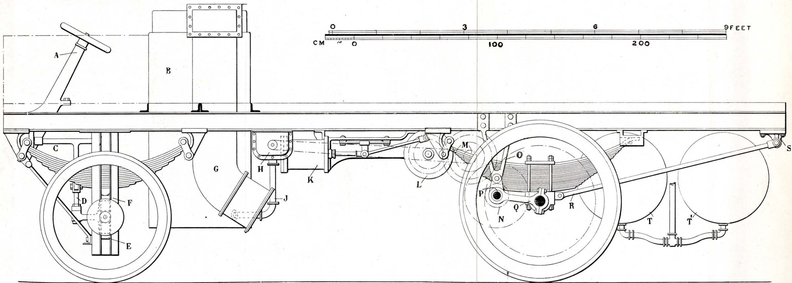
FIG. 365.—HERSCHMANN'S 5-TON STEAM WAGON.—ELEVATION.
