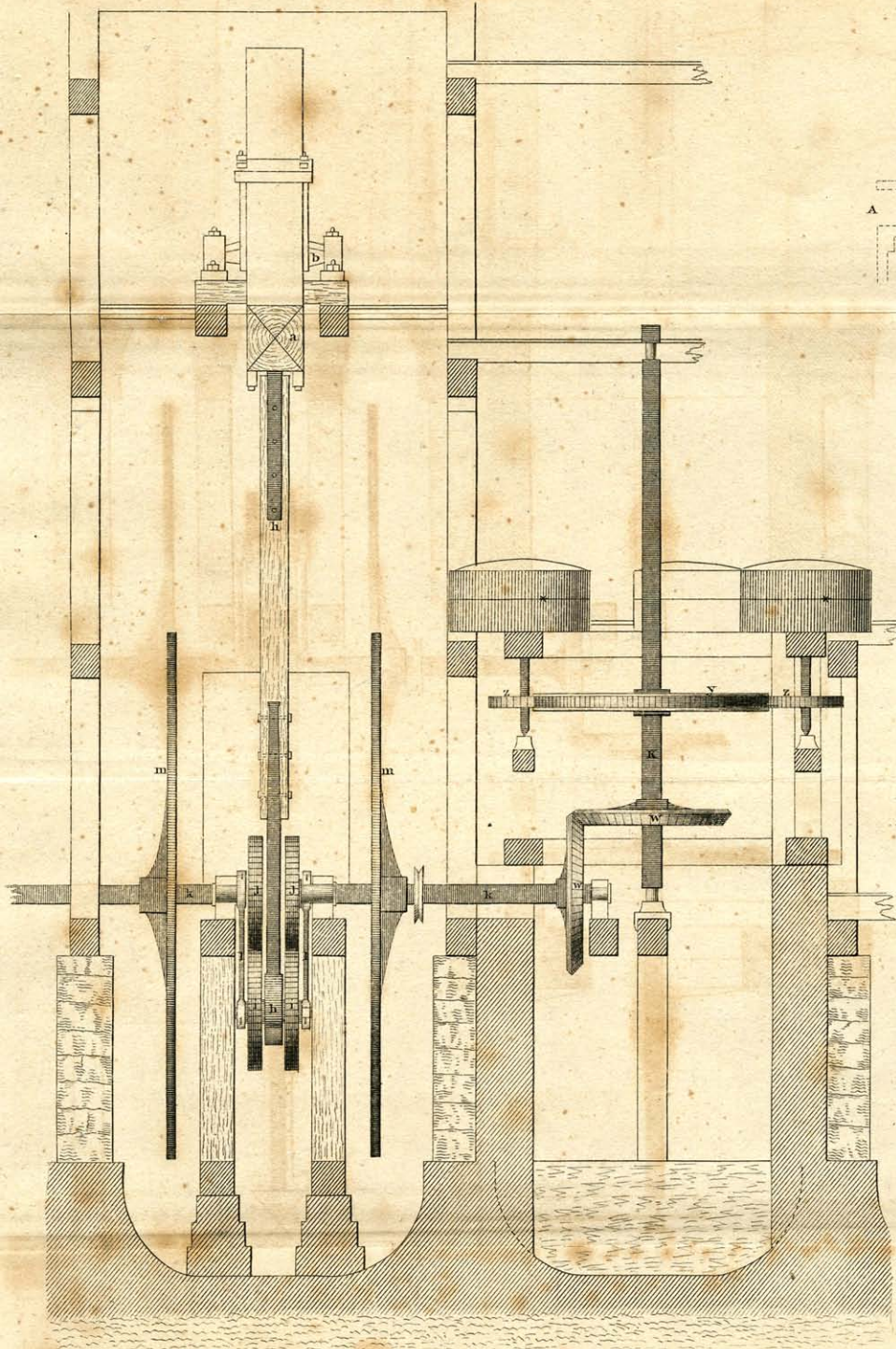
EDGE VIEW of the ROTATIVE MOTION of ONE of the ALBION MILL ENGINES.
