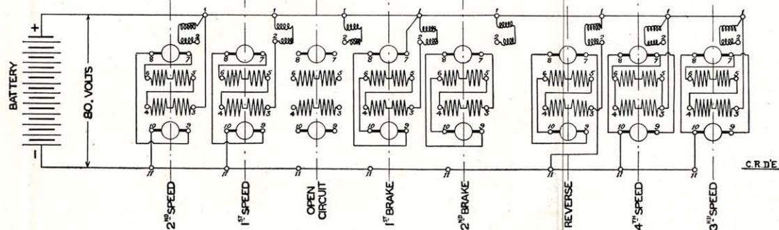
FIGS. 289-294.—PLAN, END VIEW, DEVELOPMENT AND DETAILS ON CONTROLLER OF LONDON ELECTRIC CAB.
