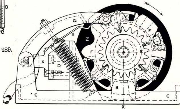
FIGS. 289-294.—PLAN, END VIEW, DEVELOPMENT AND DETAILS ON CONTROLLER OF LONDON ELECTRIC CAB.
