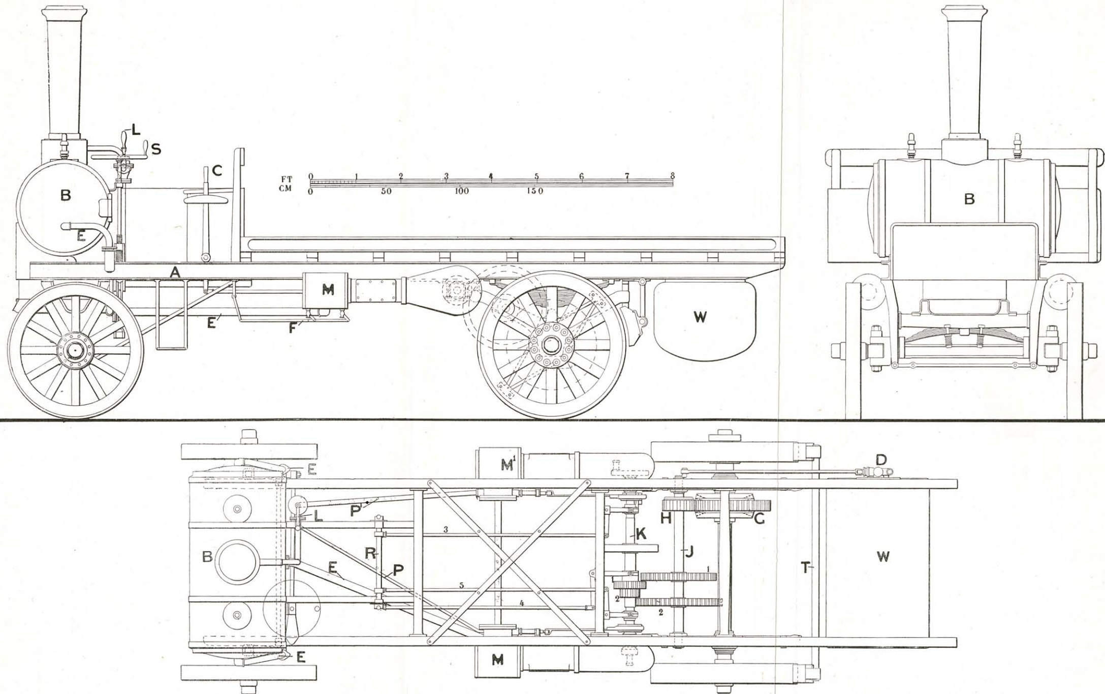
FIGS. 358, 359-360.—ELEVATION, FRONT END VIEW, AND PLAN OF YORKSHIRE STEAM WAGON COMPANY'S 4-TON LORRY.
