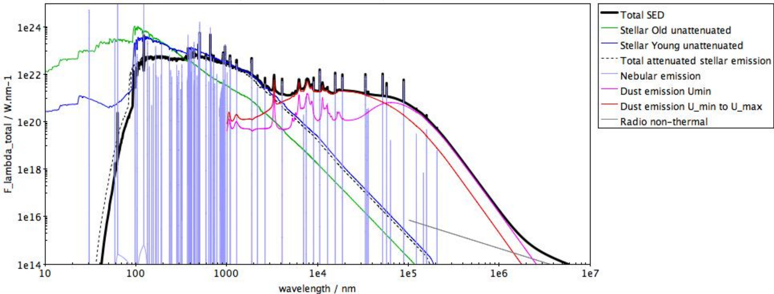
Messier 82 fitted by CIGALE with some of the components used in the fit
