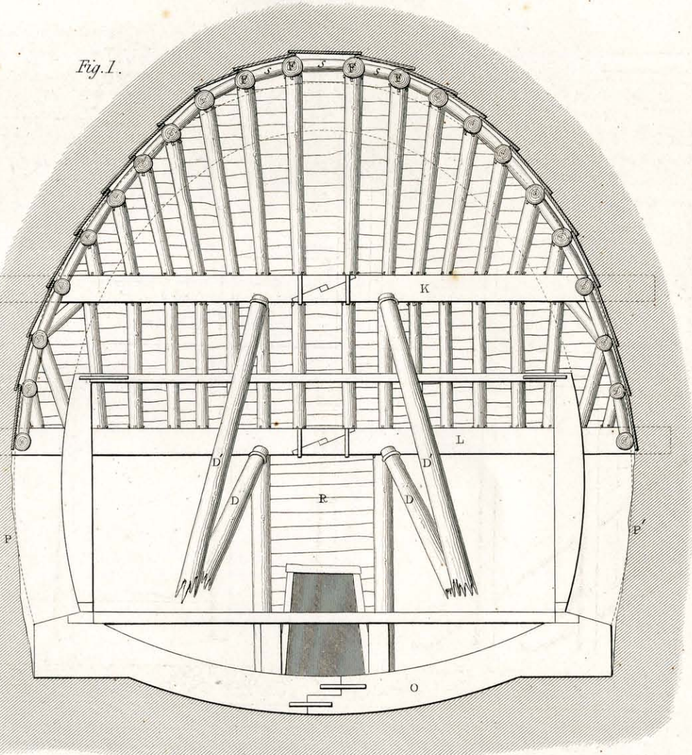
Section on line A. B.
