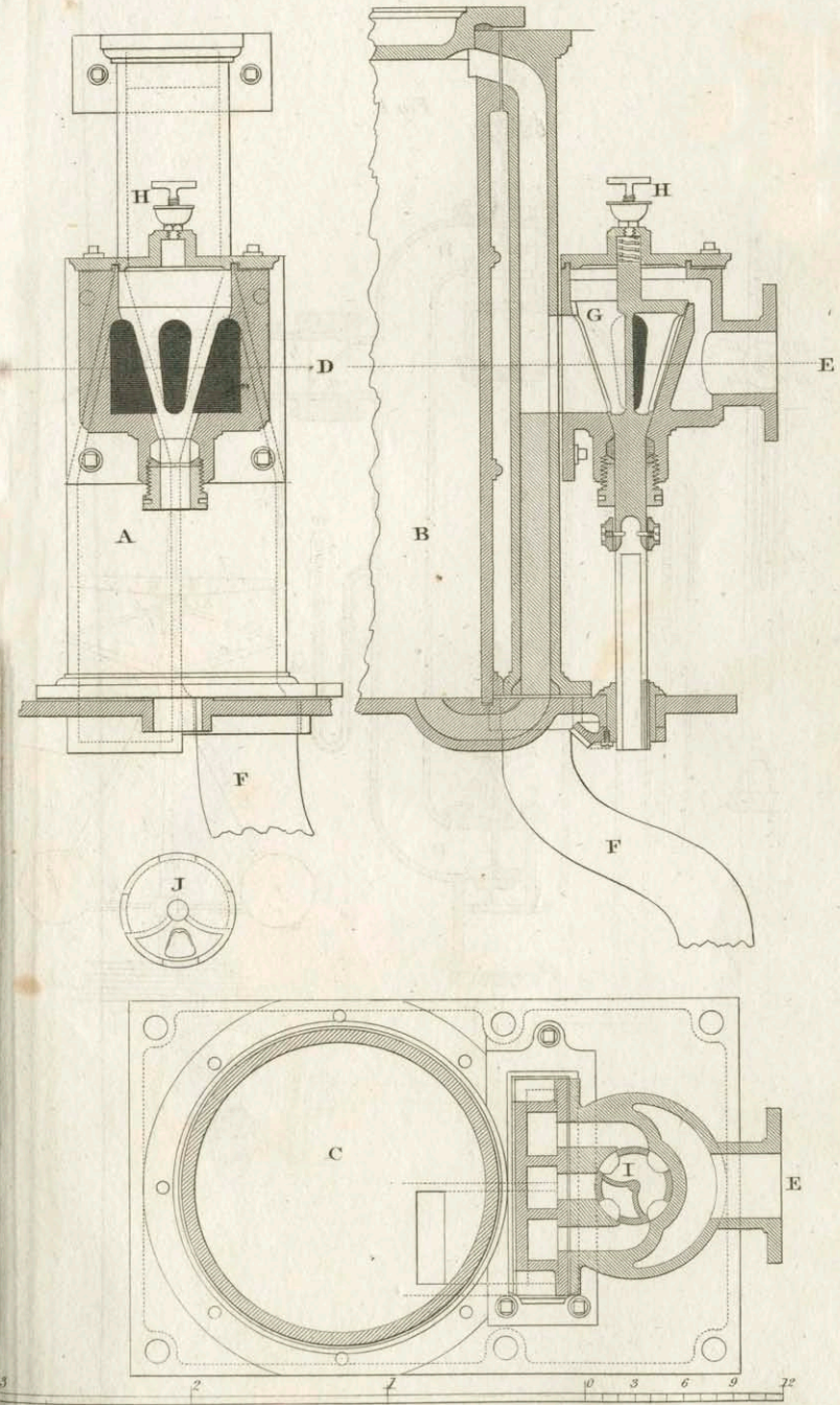
Section of the Cylinder and working Valves to Maudslays Engine.
