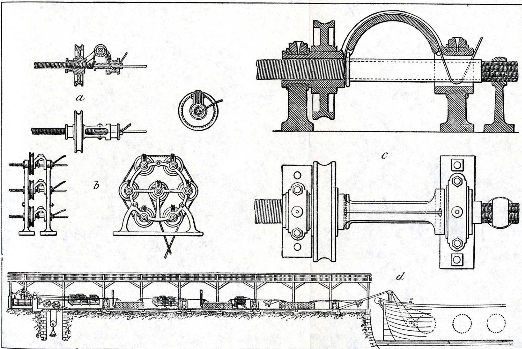
FIG. 2.—Wheatstone's Proposed Telegraph Line between England and France, 1840 (Construction and Shipment).
