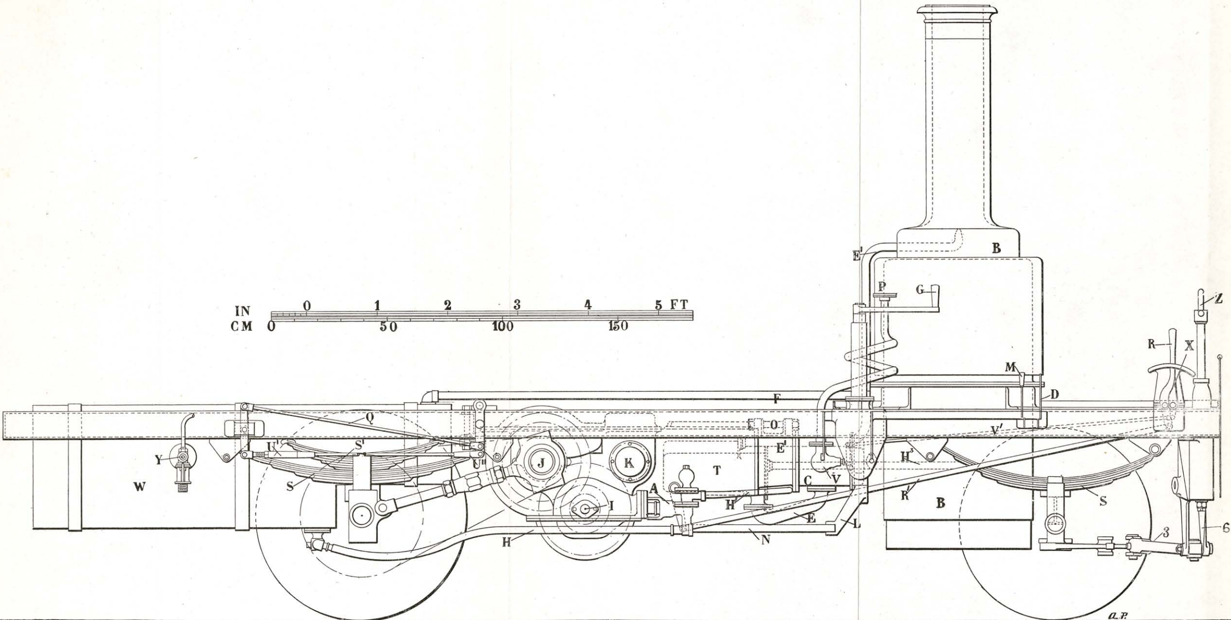
FIG. 351.—GENERAL ARRANGEMENT OF COULTHARD 5-TON STEAM LORRY.—ELEVATION.
