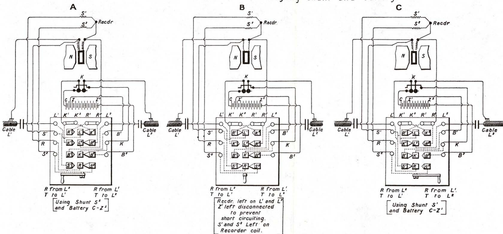
FIGS. 92 and 93.—Alternative Arrangements with Raymond-Barker's Manual Translation Switch.
