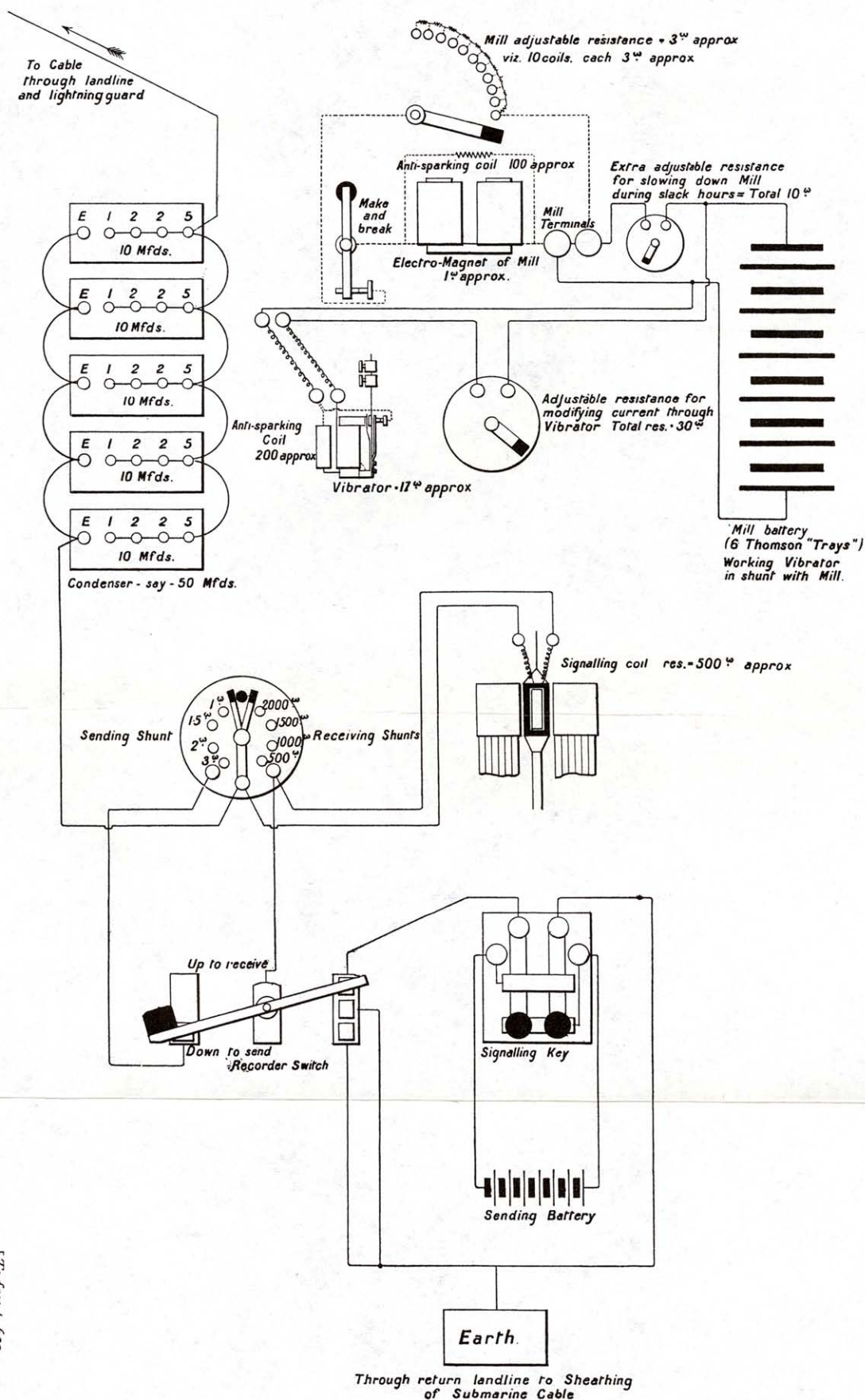
FIG. 96.—Siphon Recorder Apparatus installed at the Stations of the South American Cable Company.
