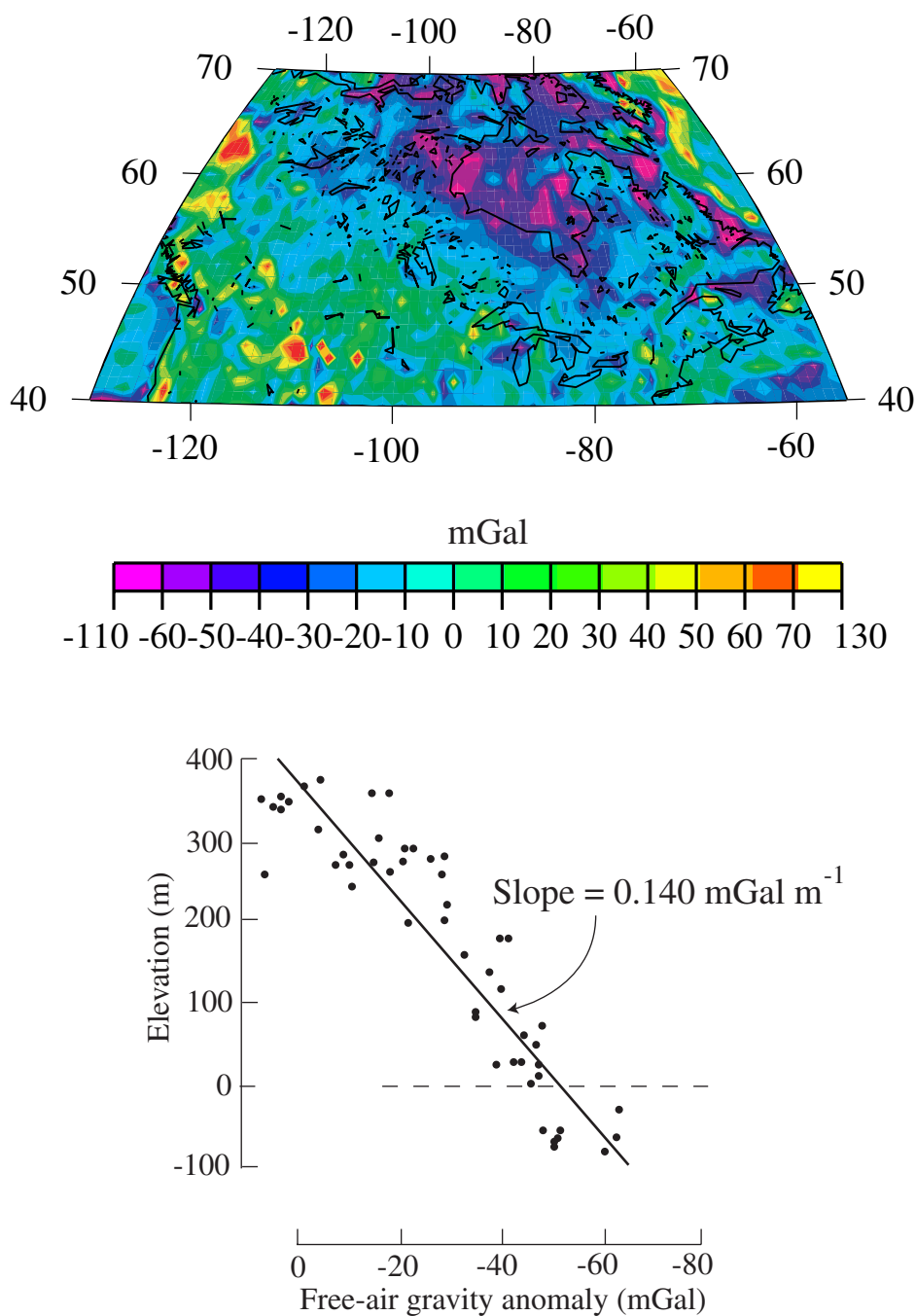
Fig. 1.30. The free-air gravity anomaly over Canada and the northern United States and its relationship to the topography. Reproduced from the Decade of North of America geophysics data set and with permission from Fig. 4 of Walcott (1970c).
