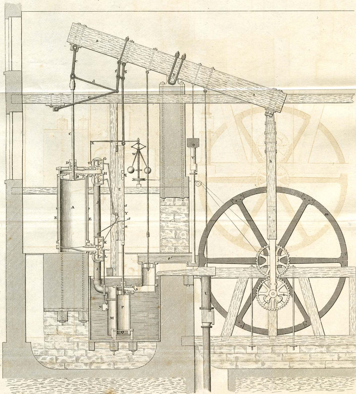
SIDE VIEW or SECTION, of ONE of the ALBION MILL STEAM ENGINES. 1787.
