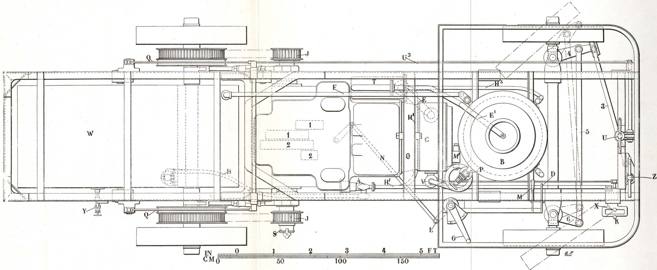
FIG. 353.—GENERAL ARRANGEMENT OF COULTHARD 5-TON STEAM LORRY.—PLAN.
