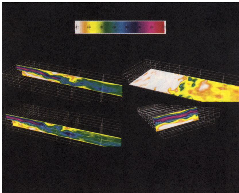
Plate 1 Color contours of instantaneous streamwise velocity along the span, on a horizontal plane, and on a vertical plane downstream of the step [ Re = 8,888 ] (see Chapter 8).
