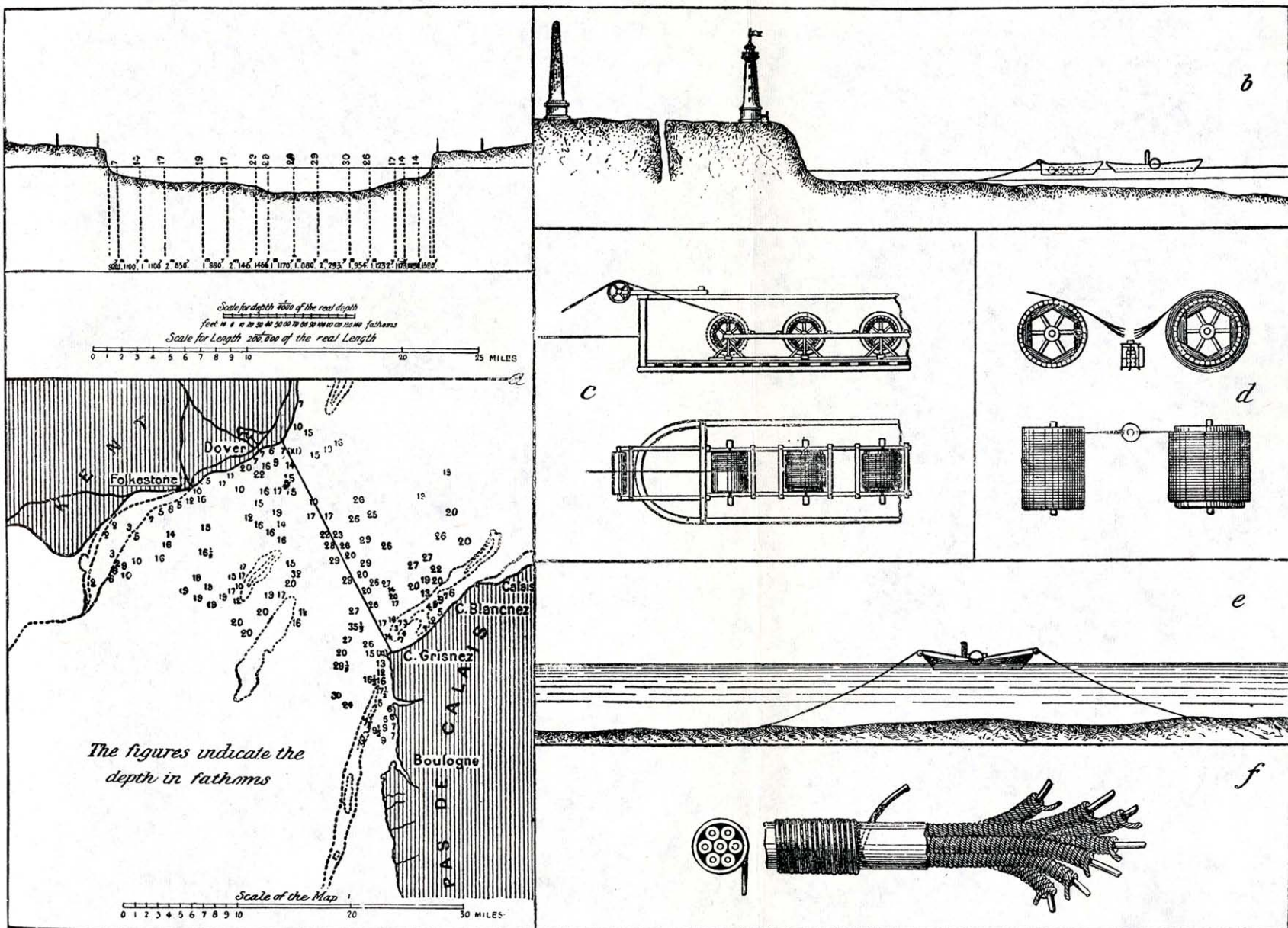
FIG. 3.—Wheatstone's Proposed Telegraph Line between England and France, 1840 (Submergence, Jointing, Underrunning, etc.).
