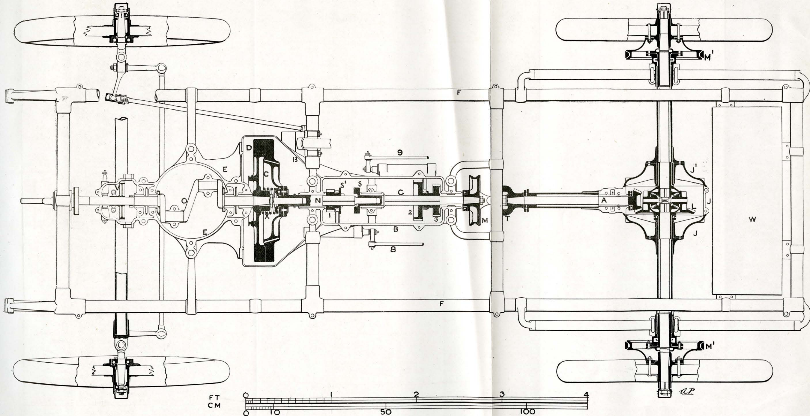
FIG. 128 —THE 10-HP. DECAUVILLE PETROL CAR: SECTIONAL PLAN OF MACHINERY, 1902-3 TYPE.
