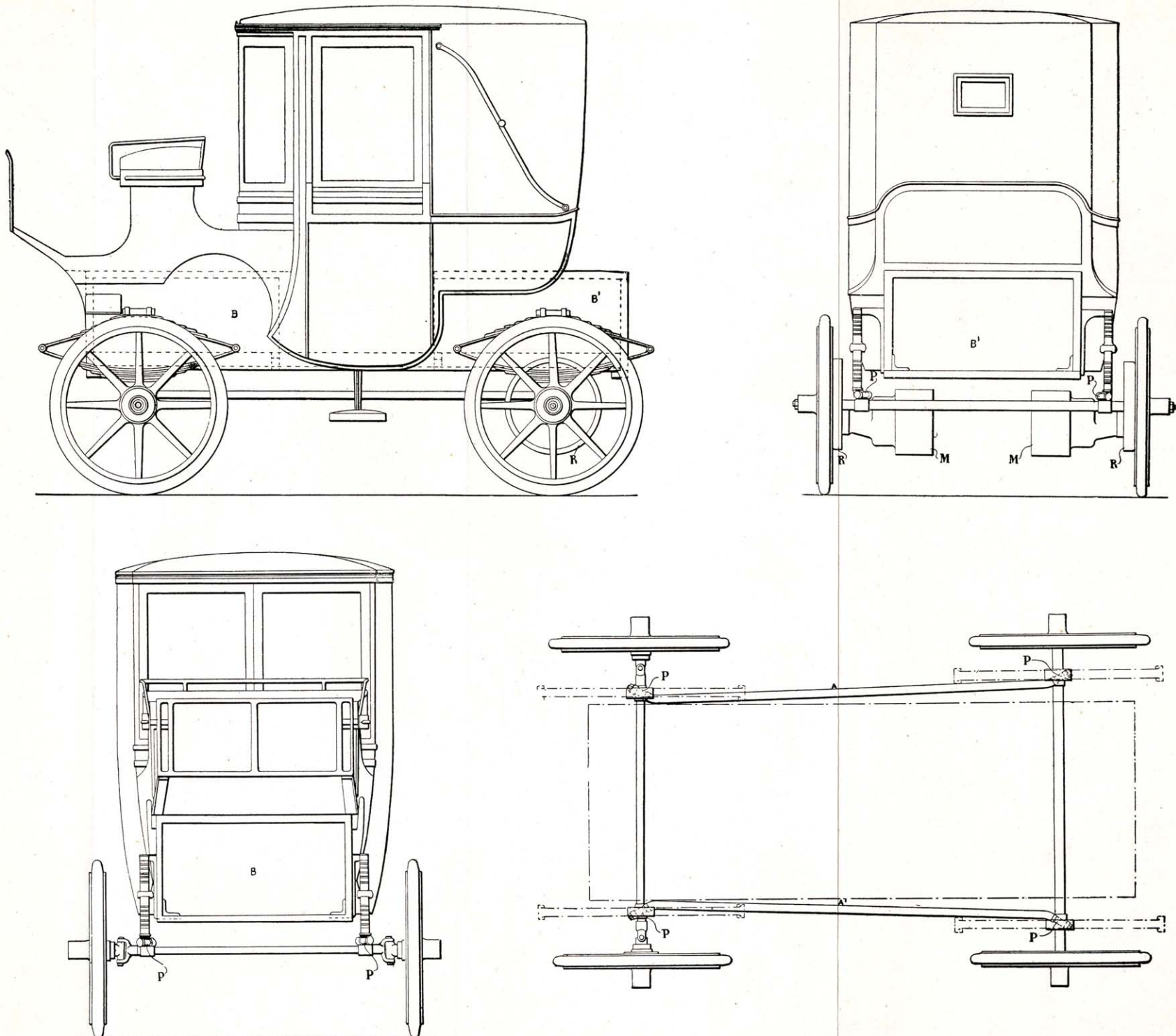
FIG. 443.—THE CITY AND SUBURBAN ELECTRIC CARRIAGE CO.—ELEVATION AND END VIEWS OF LANDAUET AND PLAN OF FRAME.
