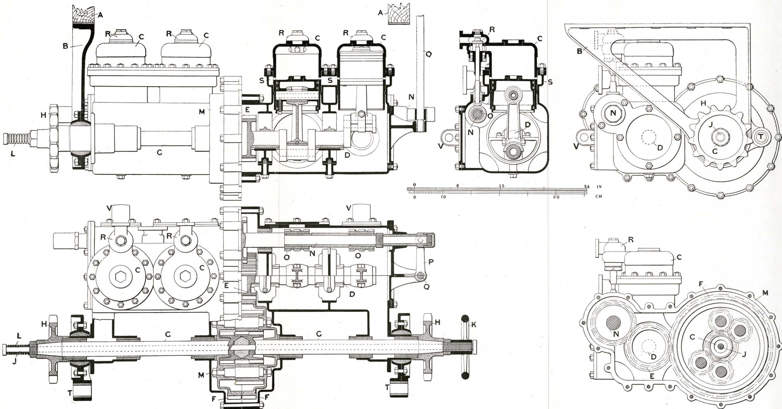
FIGS. 337 TO 341.—ENGINES, SECOND MOTION DIFFERENTIAL AND SPROCKET SHAFT OF SIMPSON AND BIBBY'S 7-TON STEAM WAGON.
