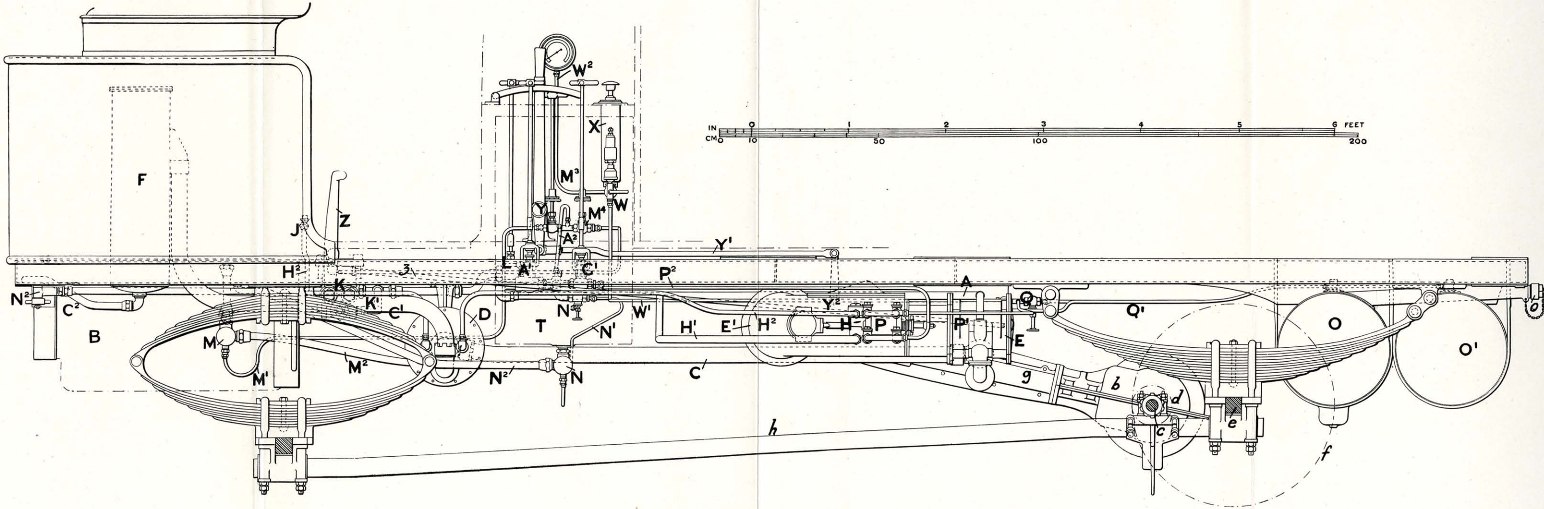
FIG. 381.—SIDE ELEVATION OF UNDERFRAME AND MACHINERY OF "LIFU" 3-TON STEAM LORRY.
