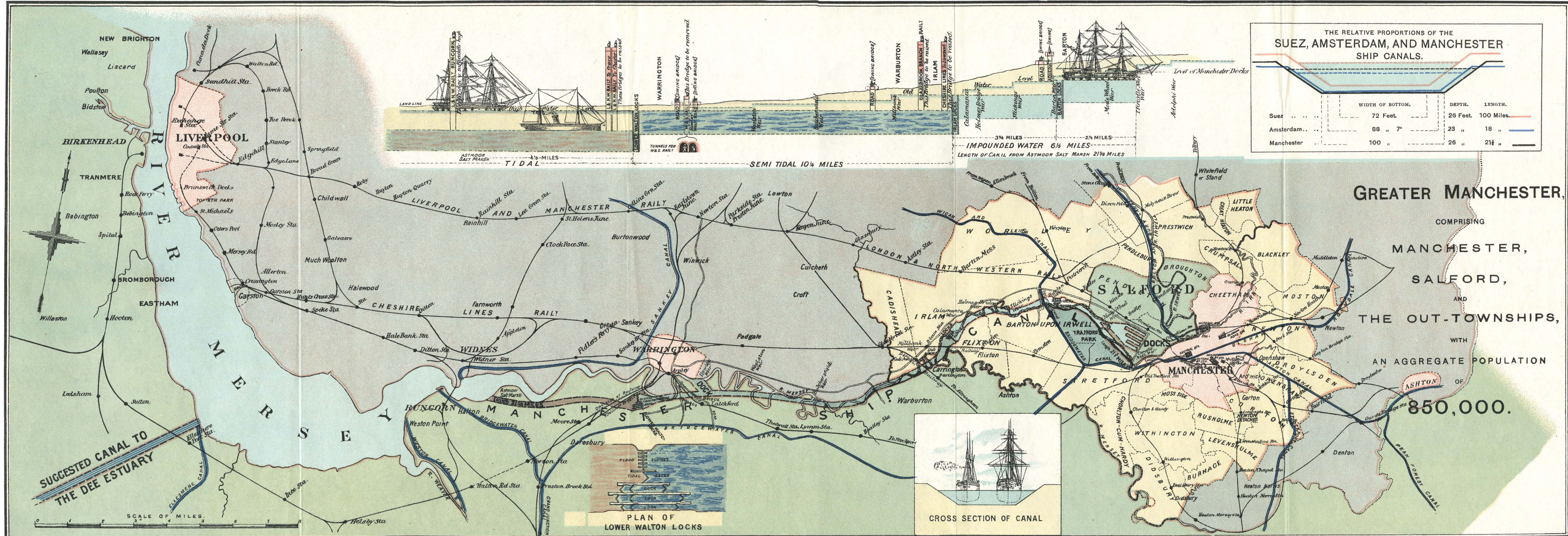
MR. BODDINGTON'S PLAN, WITH ENTRANCE AT RUNCORN AND RAILWAY PASSING UNDER CANAL; SCHEME AS APPLIED FOR IN THE BILL OF 1883.
