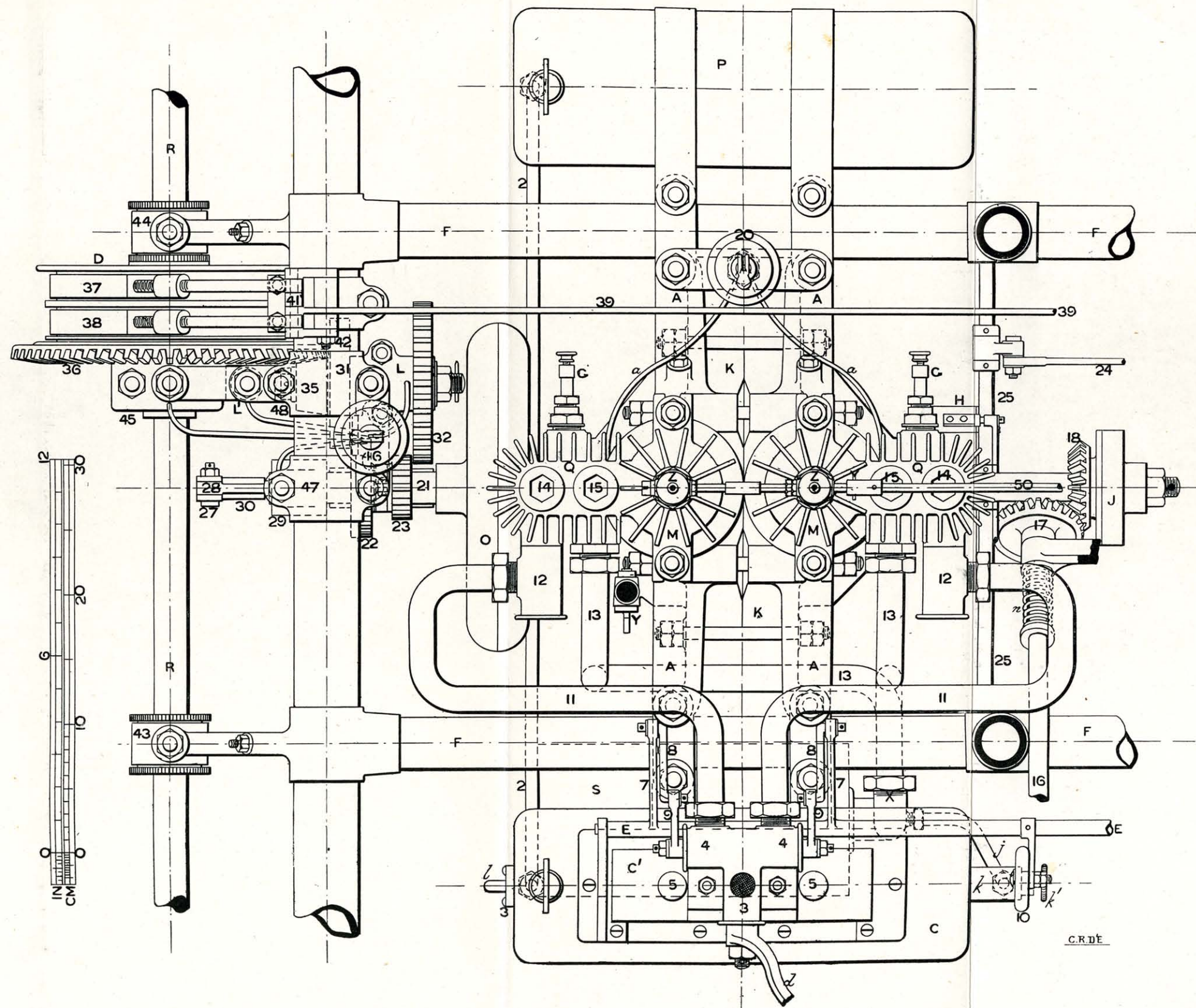
FIG. 155.—DECAUVILLE LIGHT MOTOR CAR: PLAN OF MOTOR AND MECHANISM.
