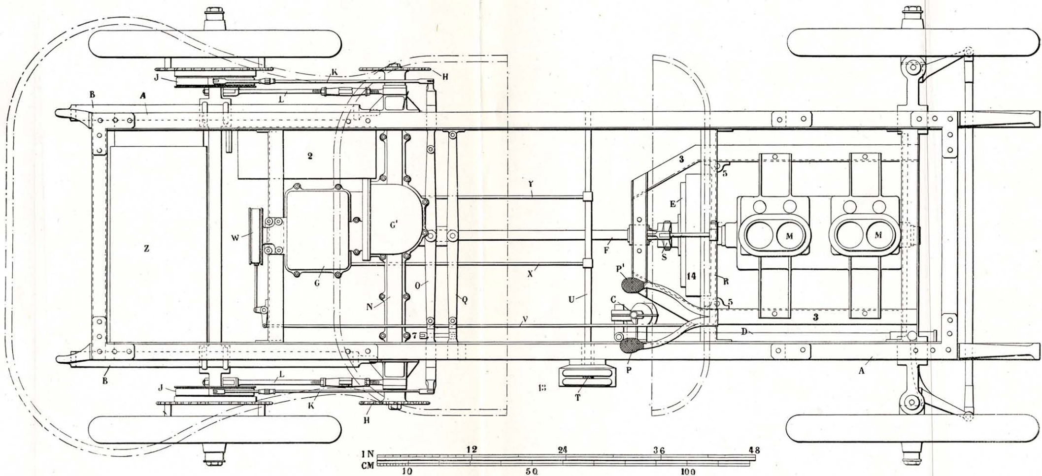
FIG. 217.—FRAME AND RUNNING GEAR OF 12-HP. DAIMLER CAR, 1902-3 TYPE.
