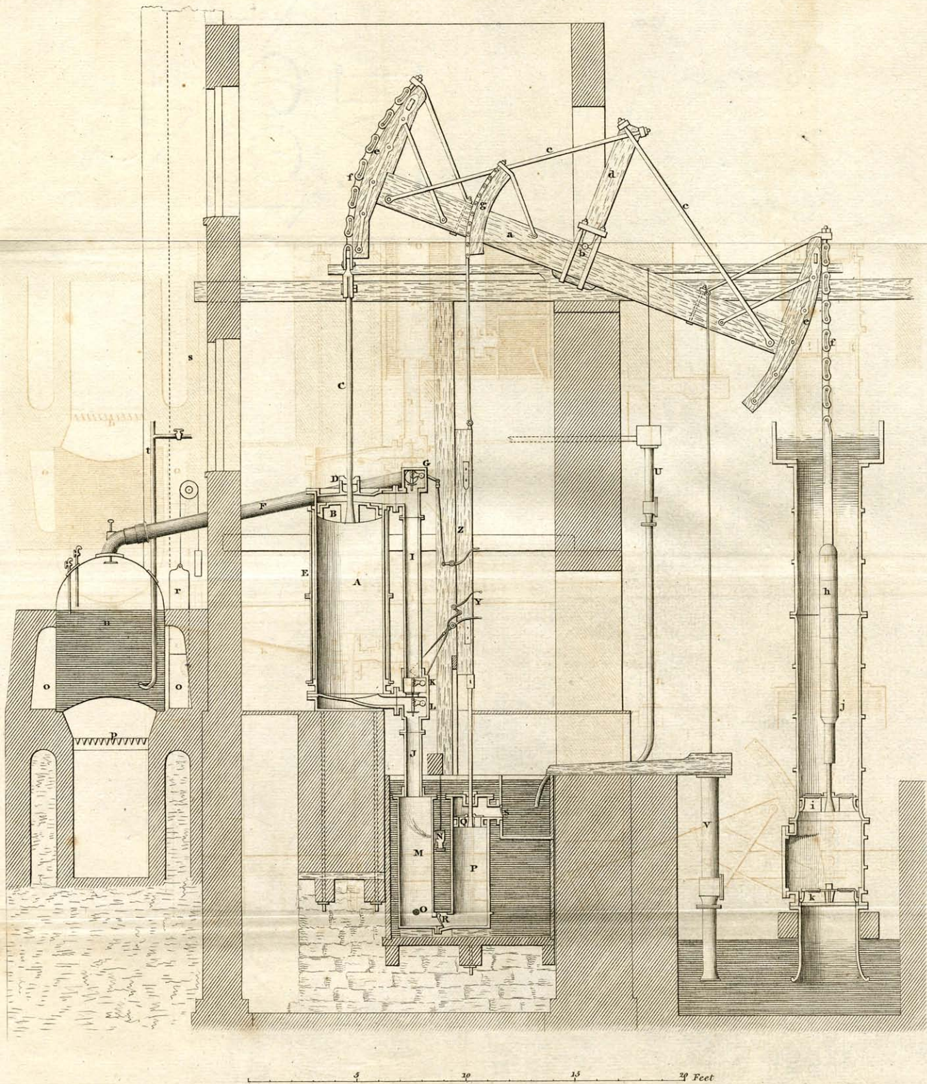
MR WATT'S SINGLE RECIPROCATING ENGINE AS CONSTRUCTED 1788.
