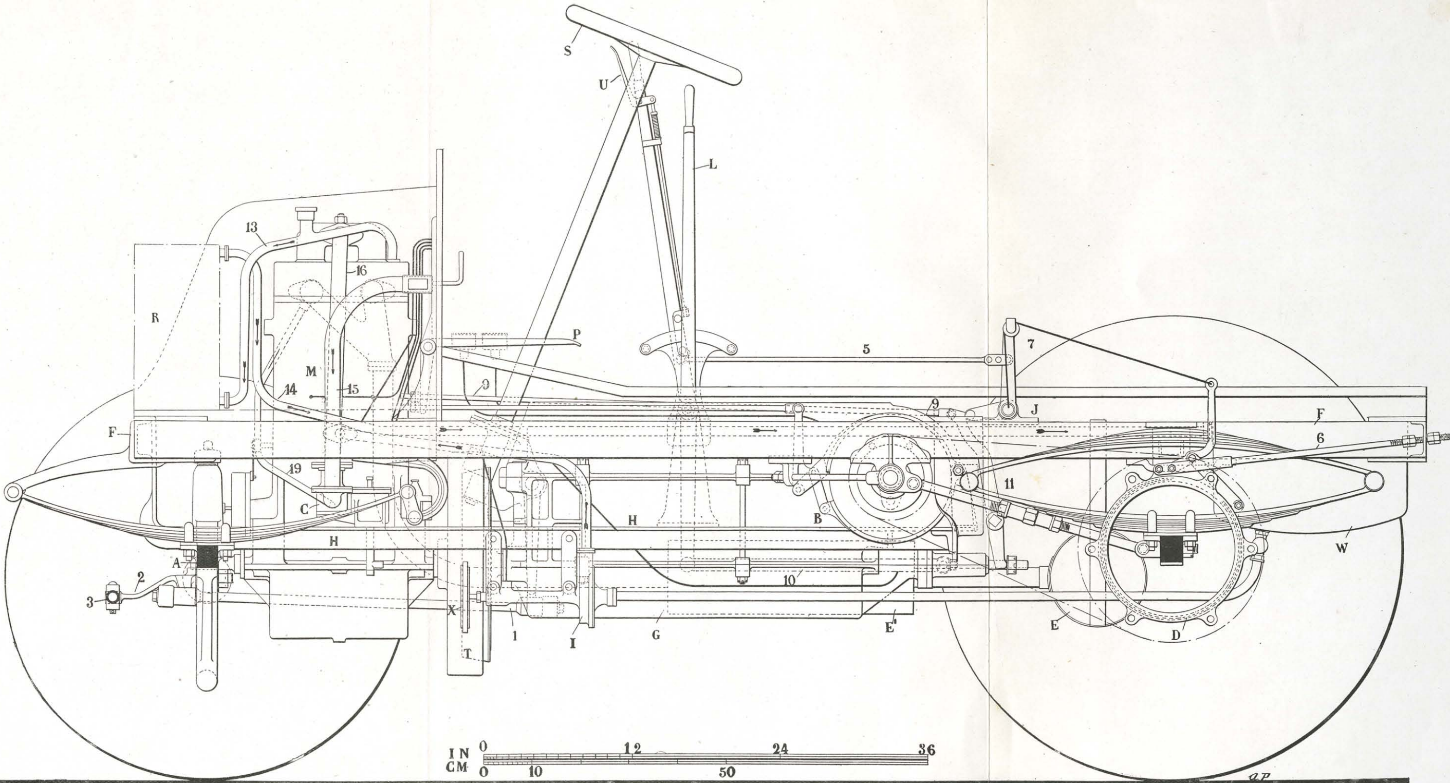
FIG. 251.—NAPIER TOURING CAR, 9 HP. 1902: ELEVATION OF FRAME AND RUNNING GEAR.
