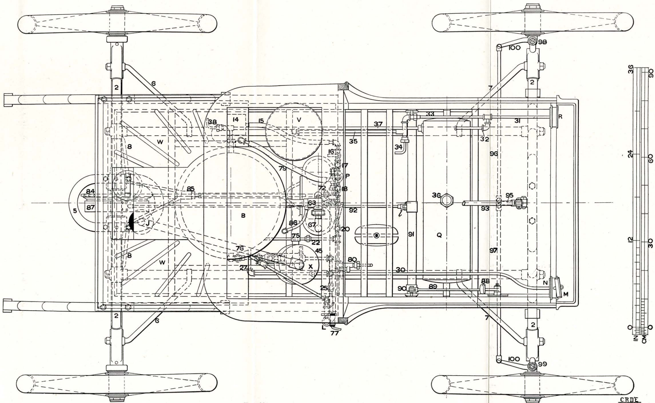
FIG. 339.—THE STANLEY LIGHT STEAM CARRIAGE: PLAN.
