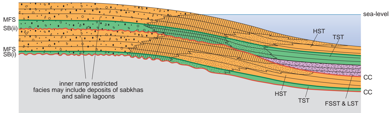
(b) arid climate evaporitic ramp
