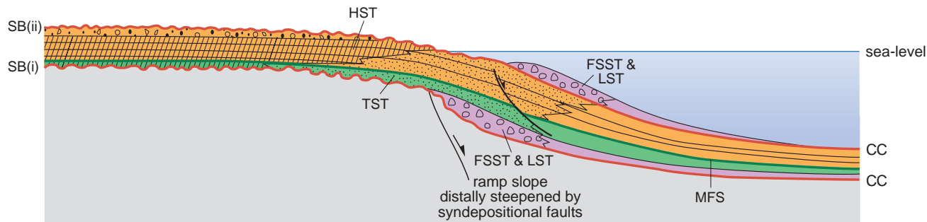
(a) distally steepened ramp
