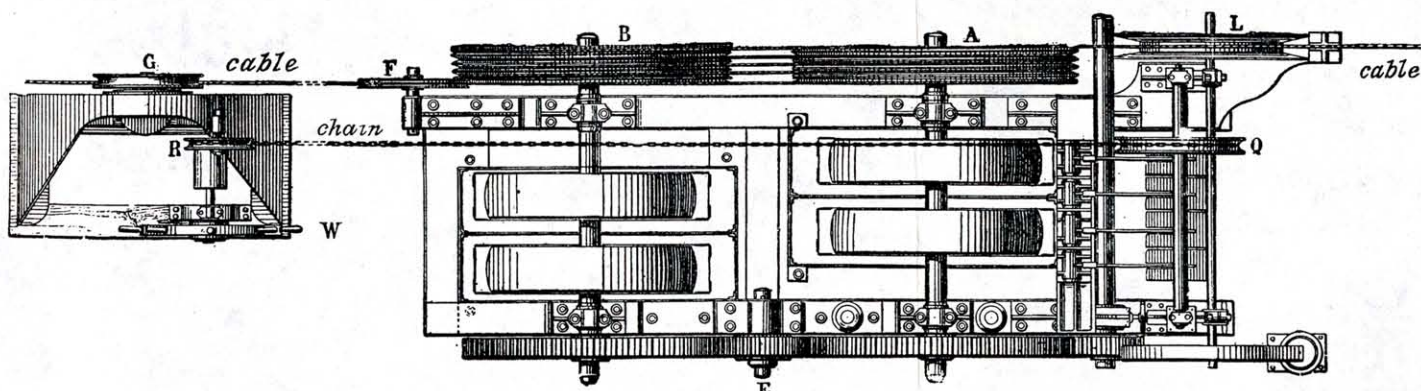
FIGS. 18, 19, 20, 21.—Paying-out Machinery of First Atlantic Cable, 1858.
