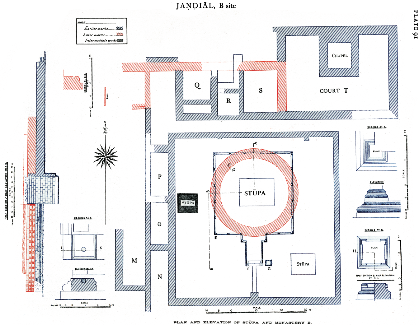
Plan, elevation and details of monastery and stūpas.
