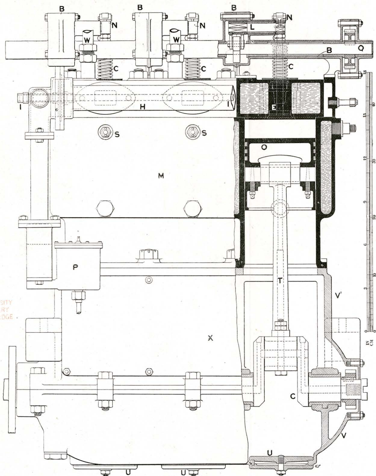
FIG. 207.—MAUDSLAY 20-HP. THREE-CYLINDER ENGINE.—SECTIONAL ELEVATION AND TRANSVERSE SECTION.
