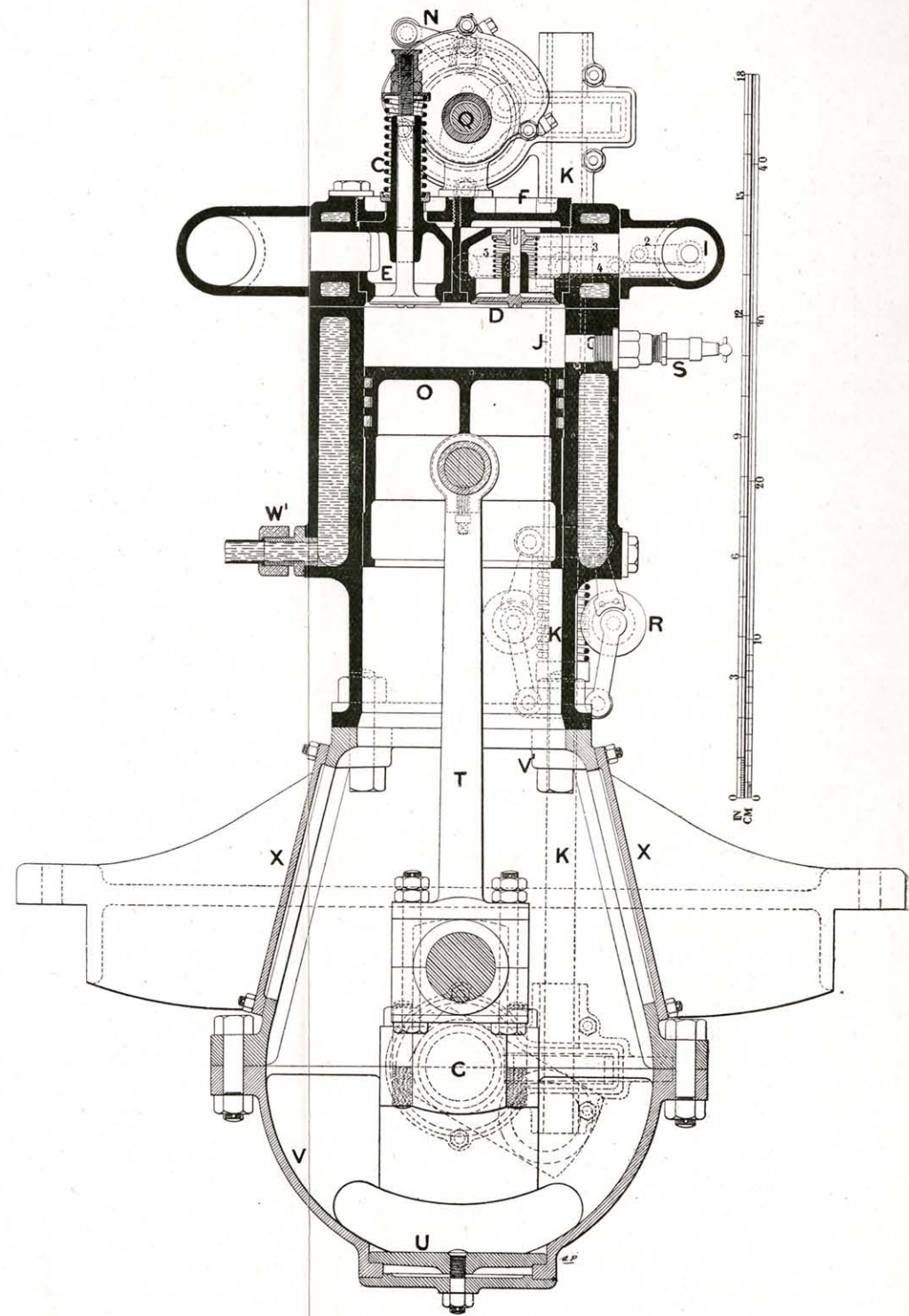
FIG. 207.—MAUDSLAY 20-HP. THREE-CYLINDER ENGINE.—SECTIONAL ELEVATION AND TRANSVERSE SECTION.
