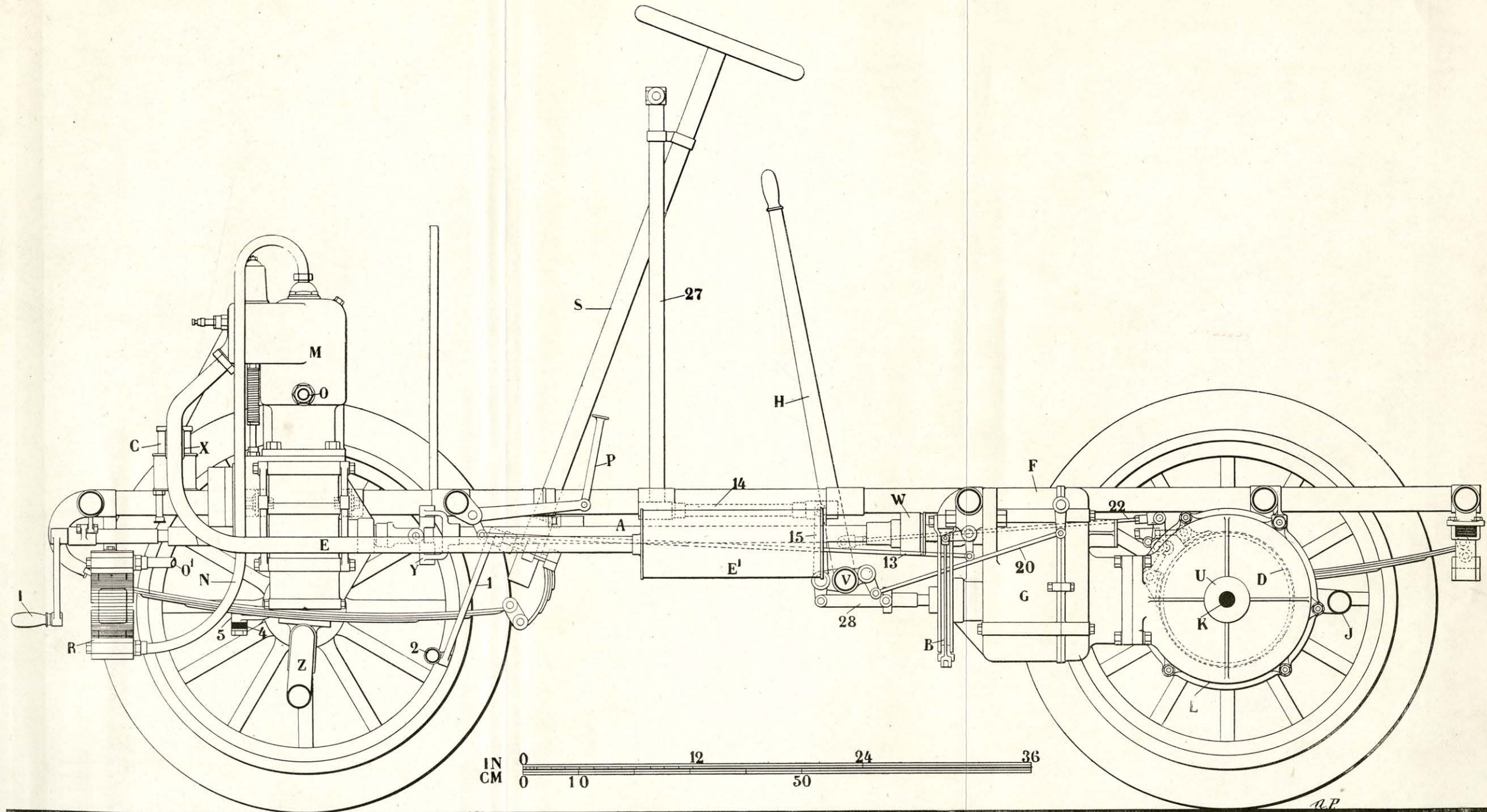
FIG. 16.—THE DE DION-BOUTON LIGHT CAR, WITH 8-HP. SINGLE-CYLINDER MOTOR.—SECTIONAL ELEVATION.
