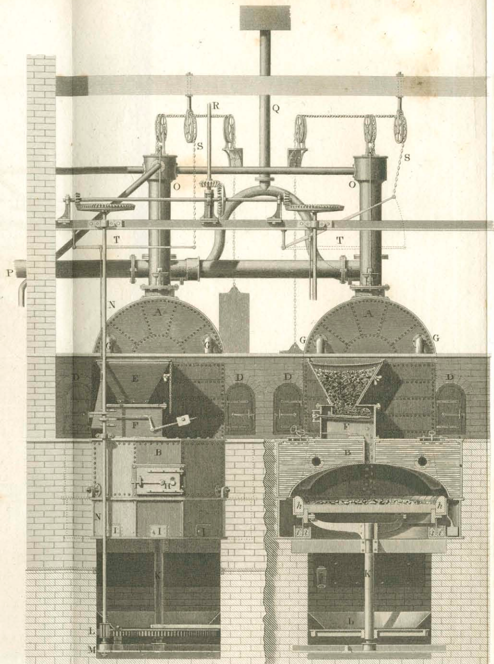
Brunton's Smoke consuming Apparatus.
