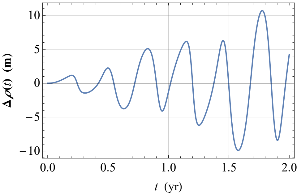
Earth–Mercury Lense–Thirring range shift
