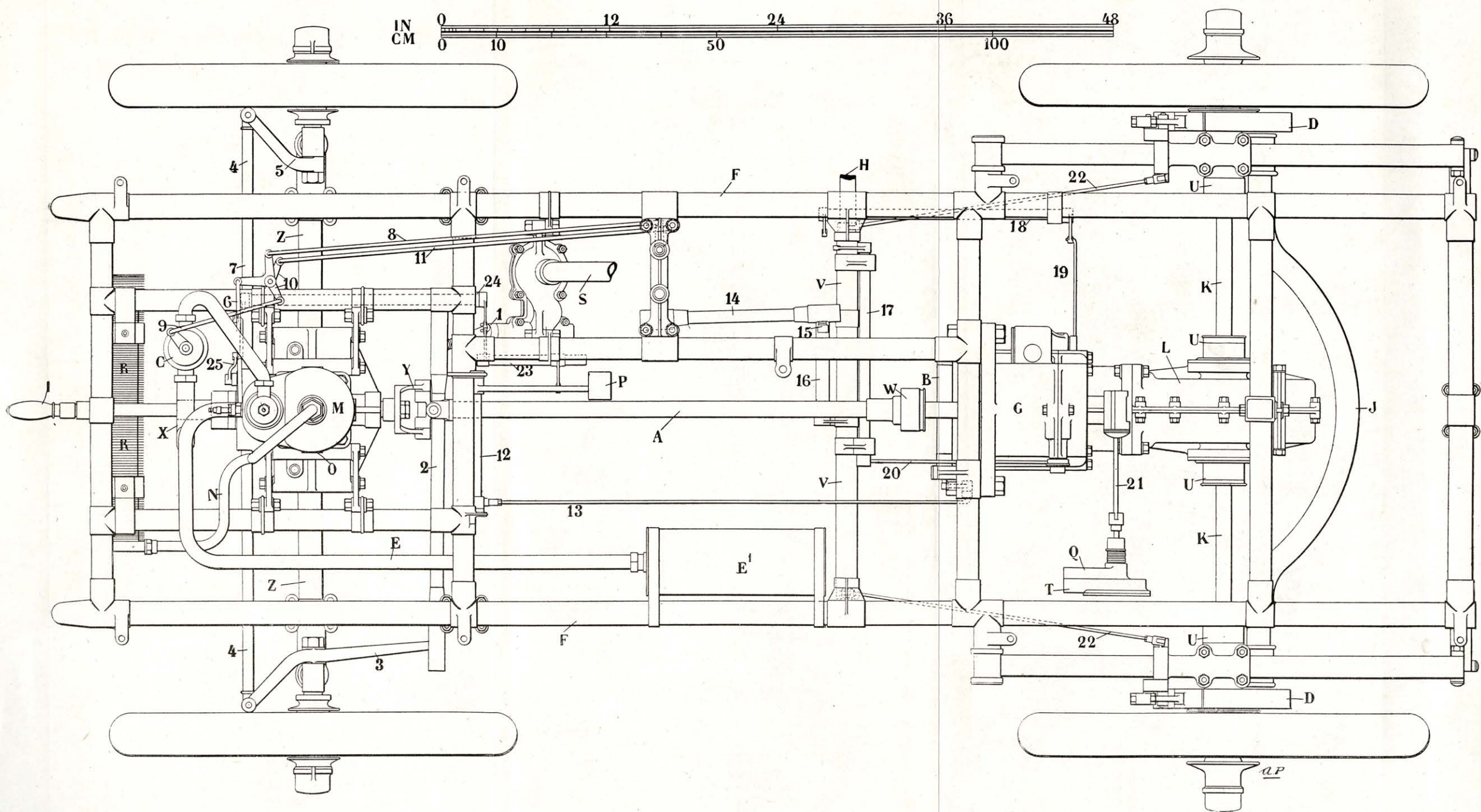
FIG. 17.—THE DE DION-BOUTON LIGHT CAR.—PLAN OF UNDERFRAME AND RUNNING GEAR.
