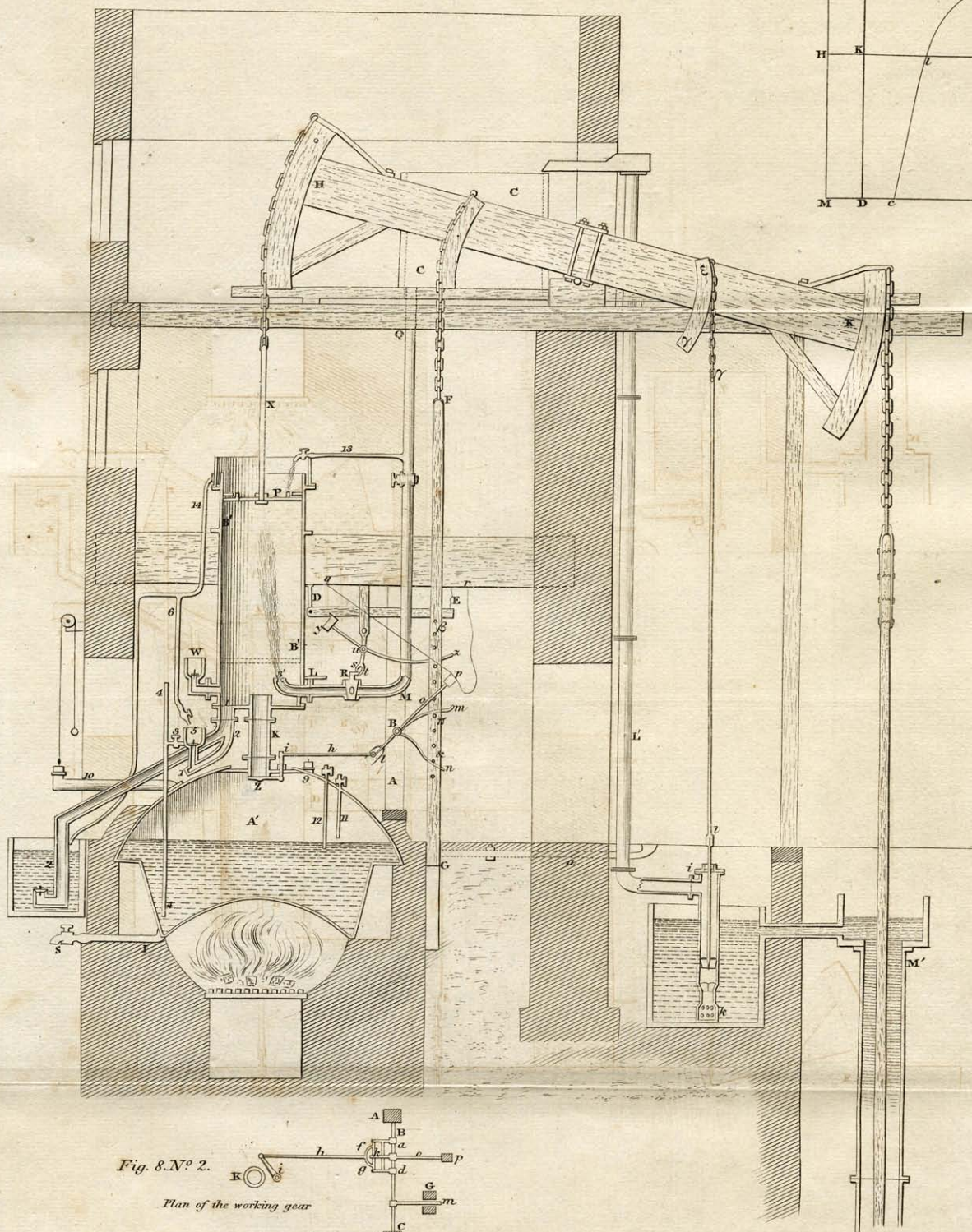
BEIGHTON'S STEAM ENGINE.
