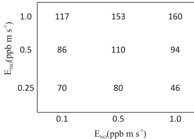
Figure AN6.3: Results of experiments 8.3.3.5: Values of ozone (in ppb) as a function of the initial emission of nitric oxide and of isoprene. For all experiments, we show the value of \text{O}_3 mixing ratio at 12 UTC.
