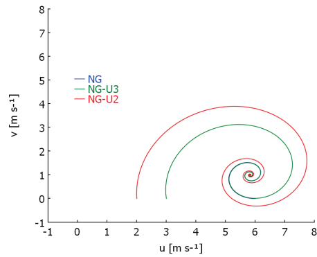
Figure AN4.3: Results of experiment 6.5.8b: Oscillation of the U and V components (trajectories) for the three experiments \langle U \rangle_0 = 6 \text{ m s}^{-1} , \langle U \rangle_0 = 3 \text{ m s}^{-1} and \langle U \rangle_0 = 2 \text{ m s}^{-1} .
