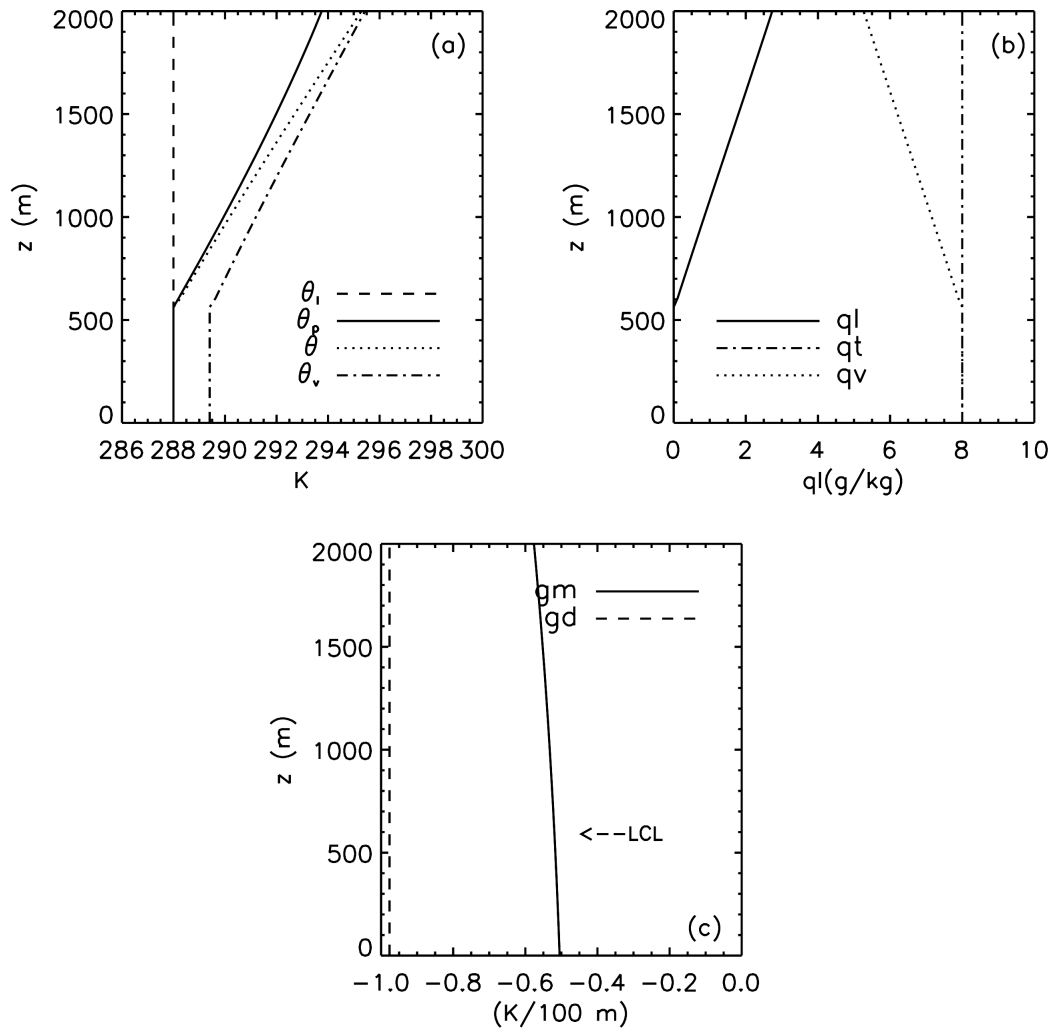
Figure AN11.2: Results of experiment 15.2: Vertical profiles of the liquid water potential temperature ( \theta_l ), potential temperature environment ( \theta ), potential temperature parcel ( \theta_p ) and virtual potential temperature ( \theta_v ) (a). Vertical profiles of the total specific humidity ( q_t ), vapour specific humidity ( q_v ) and liquid water ( q_l ) (see Box 8 for definitions) (b). Vertical profiles of the dry adiabatic lapse rate and moist adiabatic lapse rate calculated according to Equation 15.2 (c).
