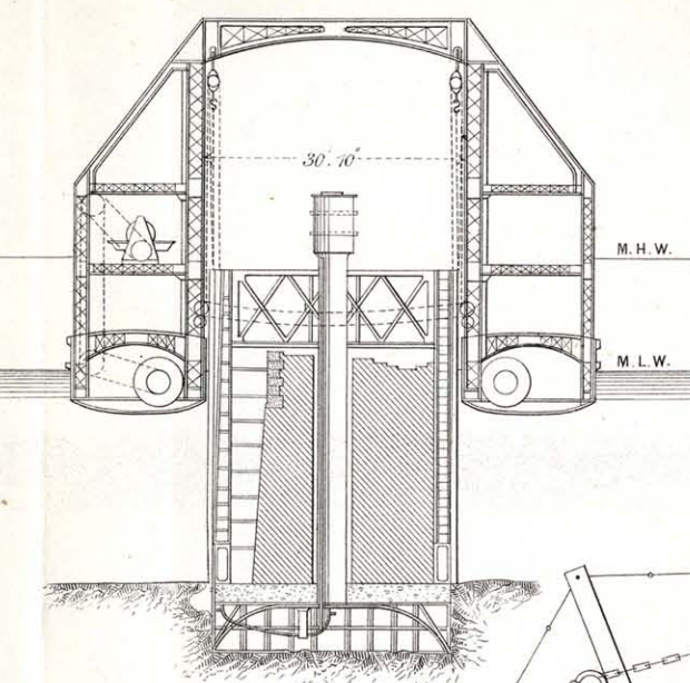
COMPRESSED AIR FOUNDATIONS ANTWERP QUAY WALLS
