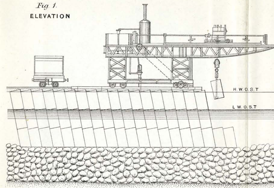
TITAN MANORA BREAKWATER.
