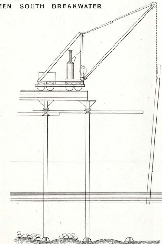
CRANES AND STAGING ABERDEEN SOUTH BREAKWATER.
