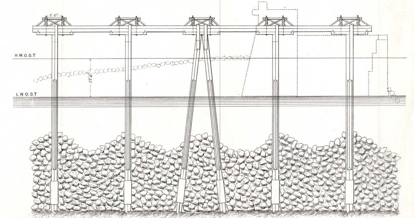
STAGING HOLYHEAD HARBOUR.
