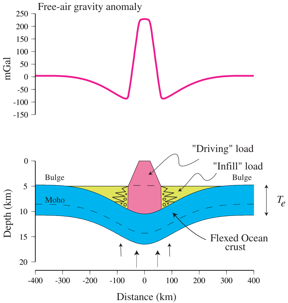
Fig. 4.15. Simple model for the gravity anomaly and flexure of the lithosphere at a seamount or oceanic island.
