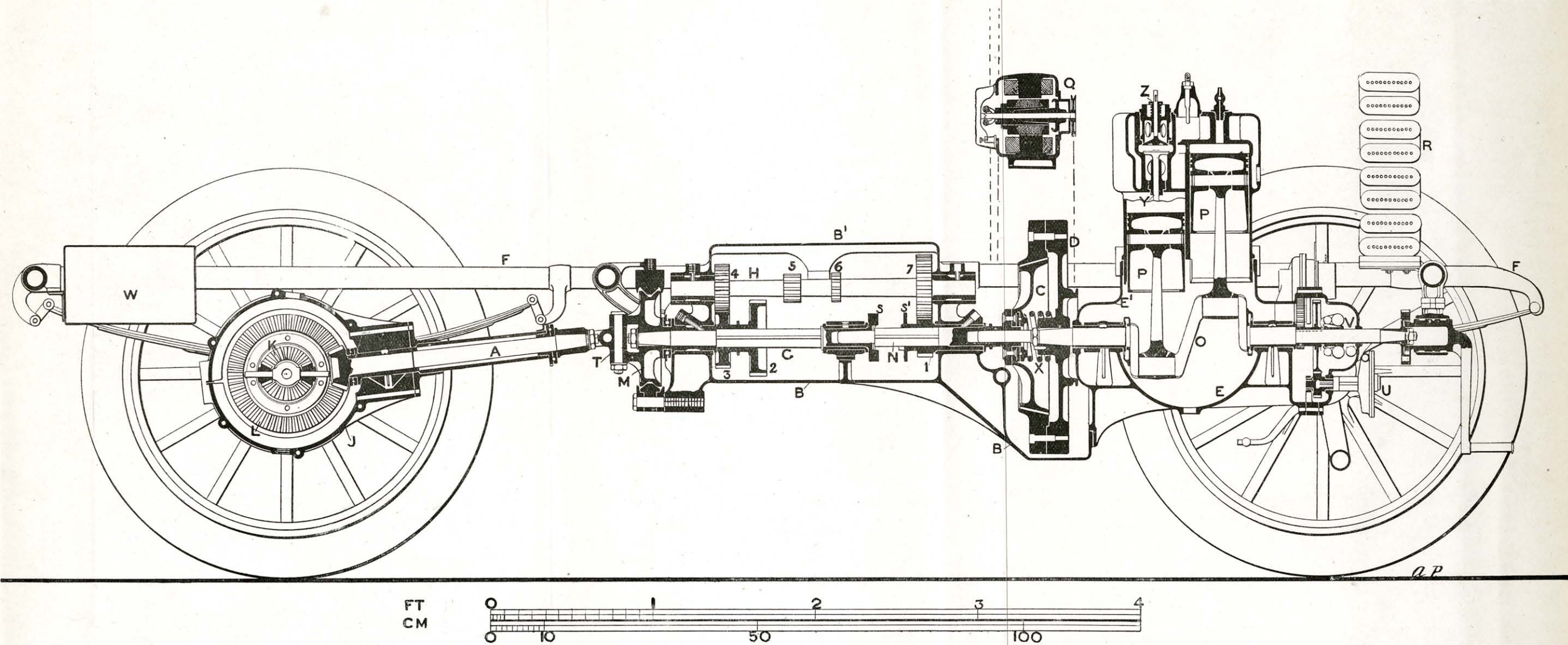
FIG. 127.—THE 10-HP. DECAUVILLE PETROL CAR.—SECTIONAL ELEVATION, 1902-3 TYPE.
