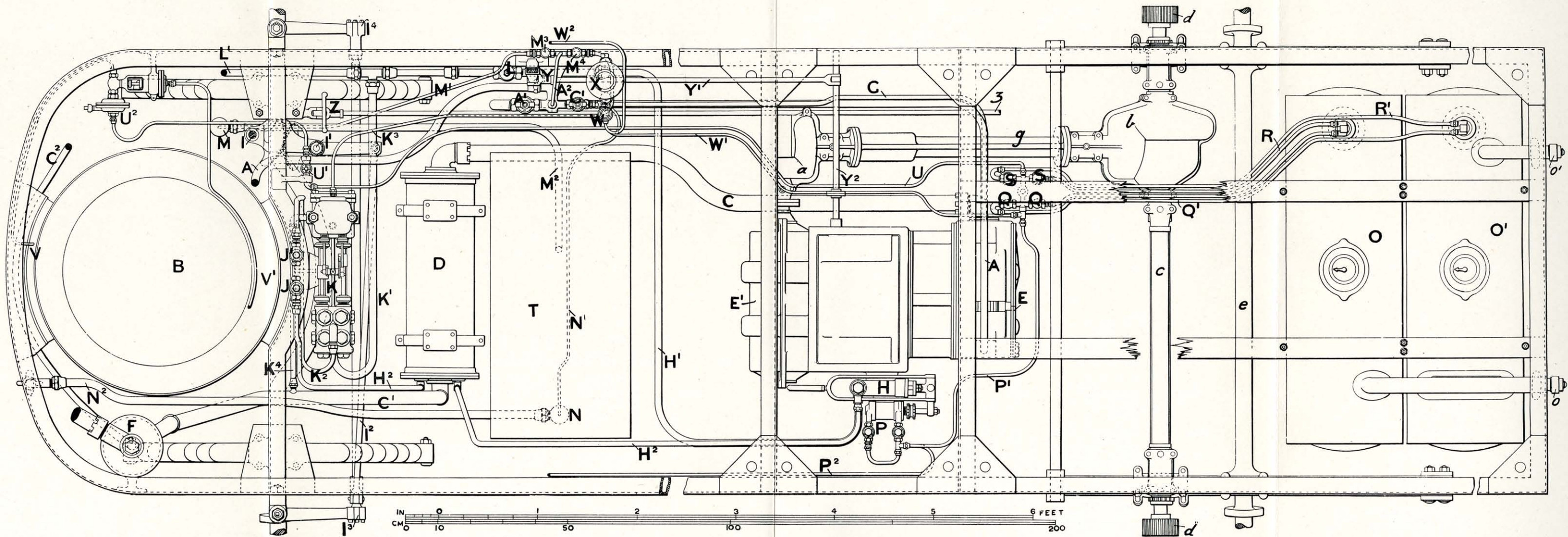
FIG. 382.—PLAN OF UNDERFRAME AND MACHINERY OF THE "LIFU" 3-TON STEAM LORRY.
