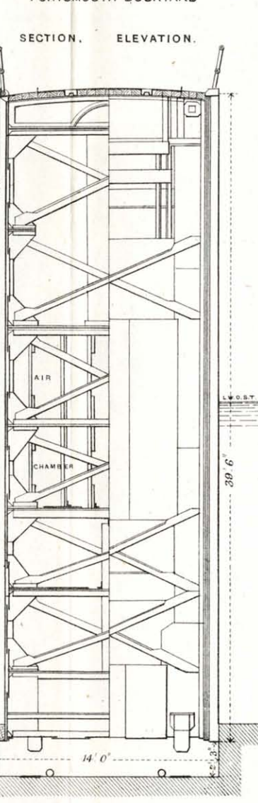
Fig. 8. SLIDING CAISSON. PORTSMOUTH DOCKYARD
