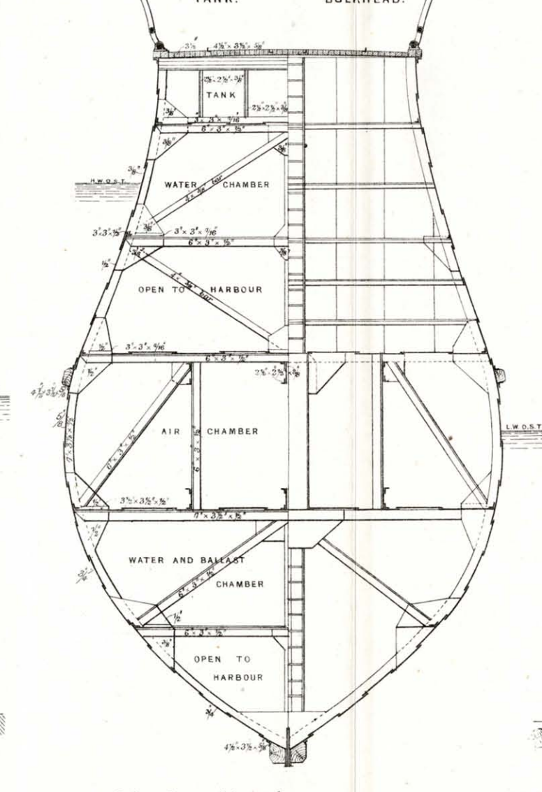
Fig. 9. SHIP CAISSON. DEVONPORT DOCKYARD
