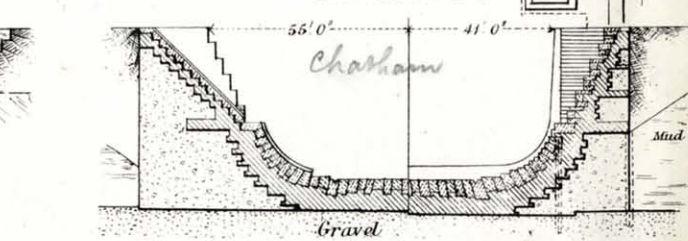
Fig. 14. SECTION ON C.C.
