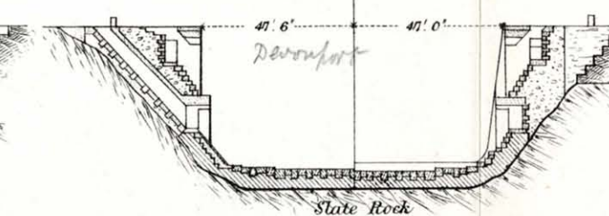
Fig. 13. SECTION ON B.B.
