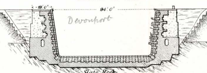
Fig. 12. SECTION ON A.A.
