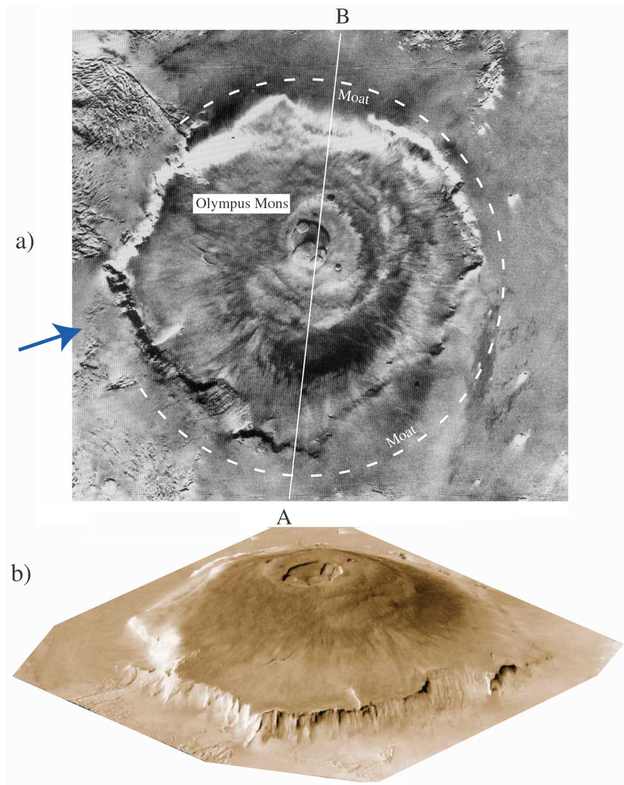
Fig. 8.15. Camera image of Olympus Mons in the Tharsis region of Mars. (a) plan view. (b) perspective view from the west. Reproduced with permission from Fig. 7.11 of Greely (1994).
