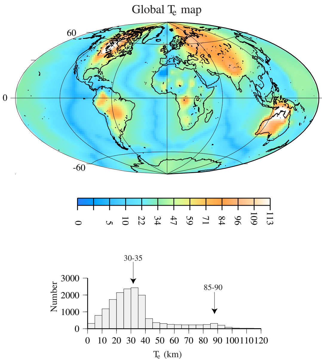
Fig. 8.30. Map of global T_e . Contours in the continents are based on selected coherence results. Contours in the oceans assume that T_e is determined by the depth of the 450°C oceanic isotherm.
