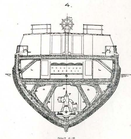
FIG. 4.—SECTION AT THE ENGINE-ROOM.
