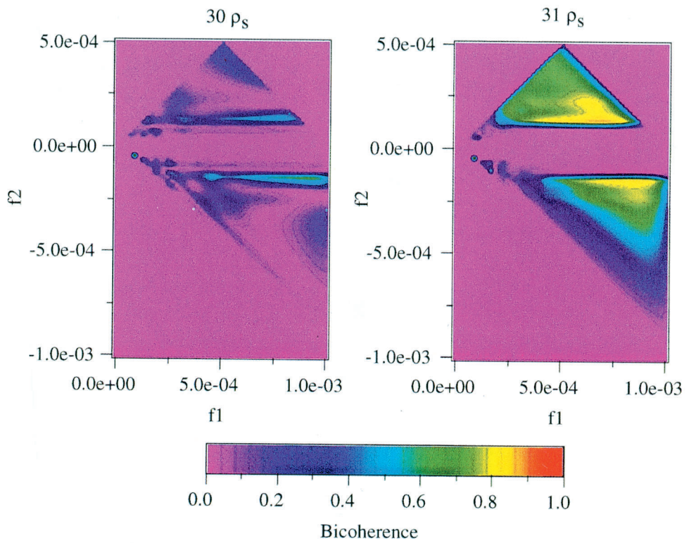
Plate 6.5f Bicoherence for r = 30.0\rho_s and r = 31.0\rho_s .
