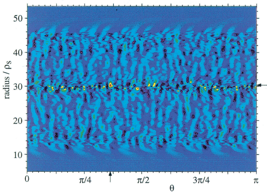
Plate 6.5e Two-dimensional graph of \tilde{n}_i in the \rho - \theta plane. The location of a small coherent structure is indicated by the arrows.
