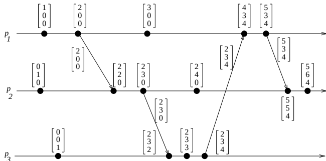
Figure 3.2: Evolution of vector time.
