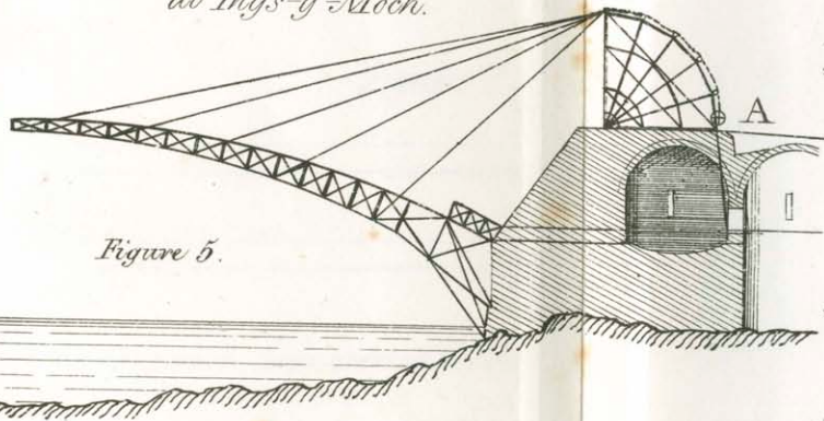
Design for the Centering of Mr Telford's Cast iron Bridge at Ynys-y-Moch.
