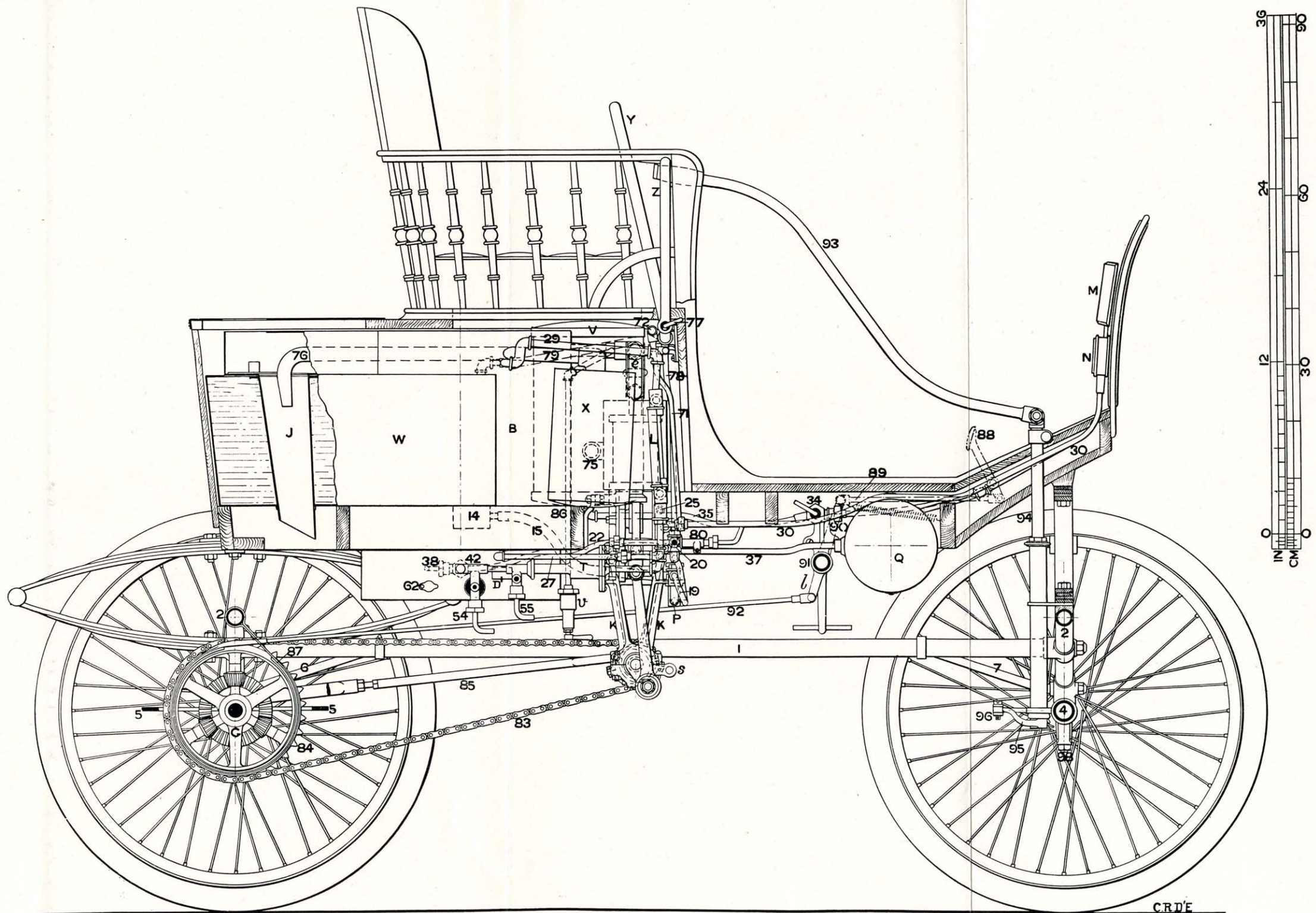
FIG. 338.—THE STANLEY LIGHT STEAM CAR: ELEVATION.
