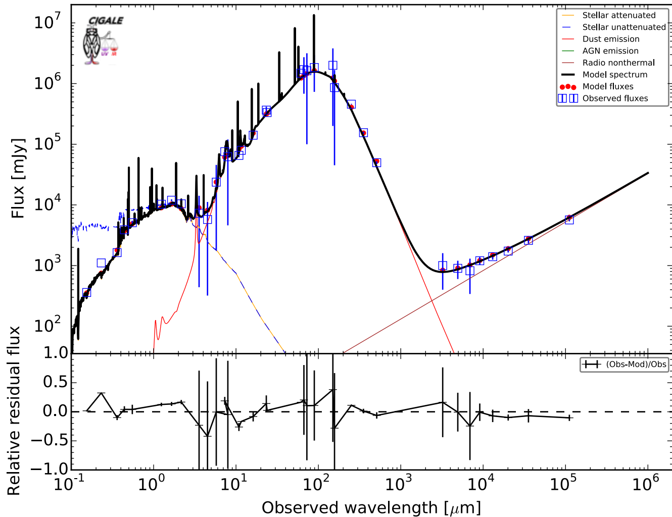
Best model for M82 at z = 0.0 . Reduced \chi^2 = 1.35
