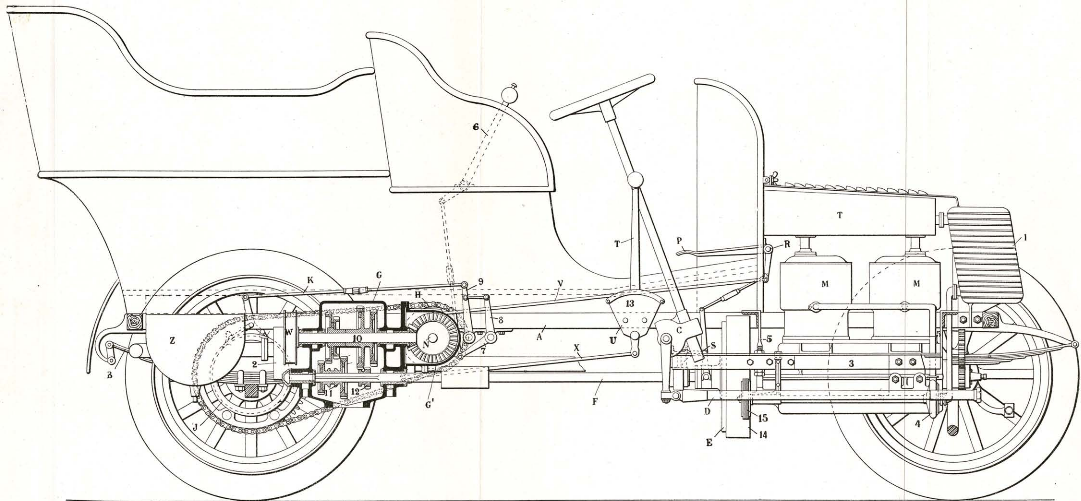
FIG. 216.—12-HP. DAIMLER TOURING CAR.—SECTIONAL ELEVATION.
